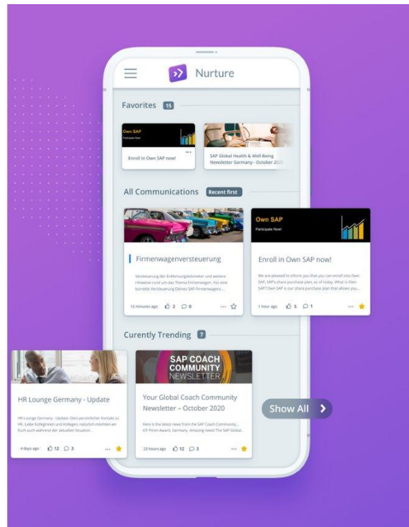
Figure 2: Mobile-friendly interface
